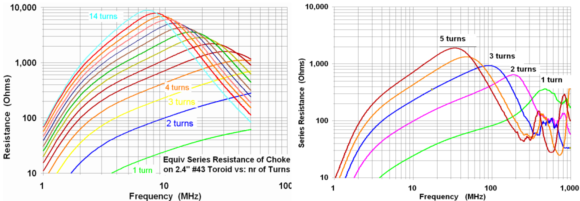
Fig 15 – Series R of chokes on the #43 2.4" toroid
