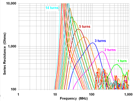
Fig 22—Series Resistance of Multi-turn chokes wound on the #61 toroid
