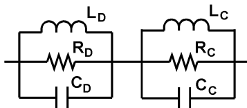
Fig 4c – A better equivalent circuit of a ferrite choke
