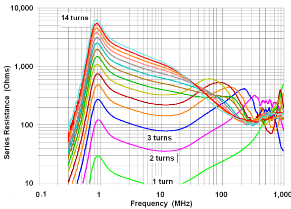
Fig 23—Series Resistance of Multi-turn chokes wound on the #78 toroid
